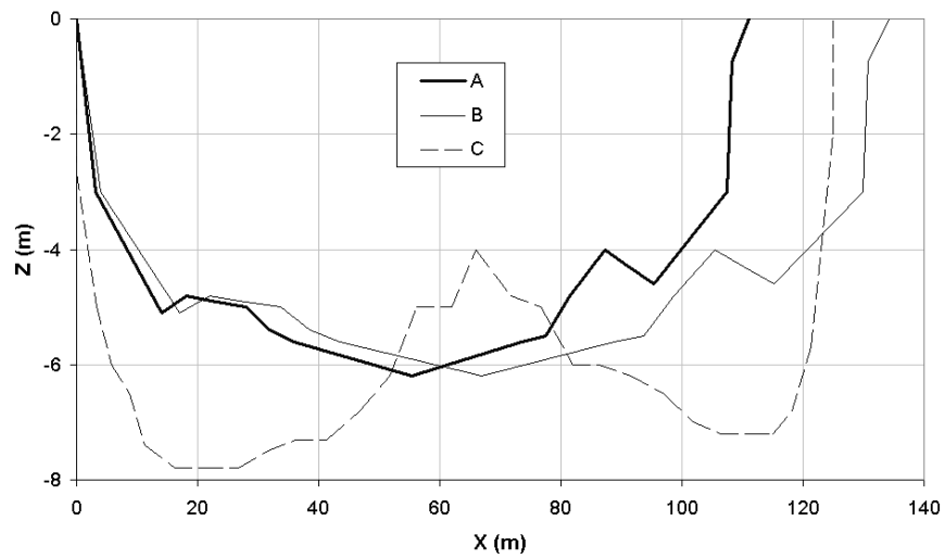
Figure 6. Cross-river profiles (Section 8).
