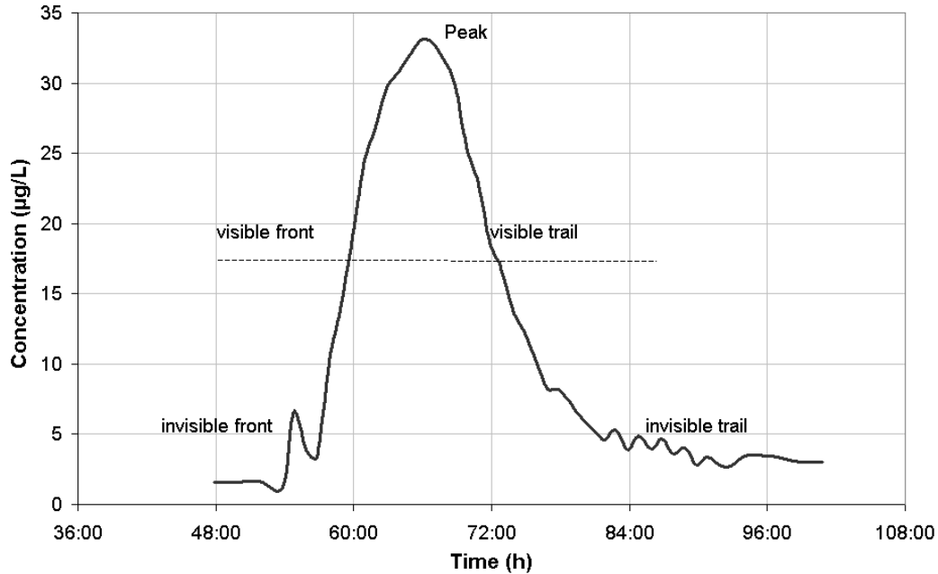
Figure 4. Characterization of tracer curves.
